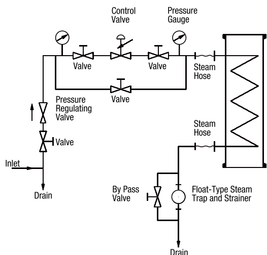
TYPICAL BOILER ARRANGEMENT
